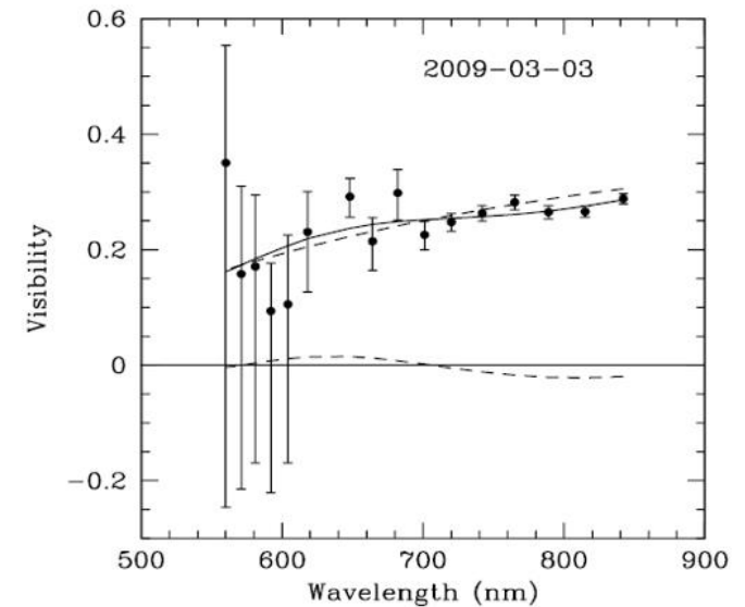
Fig. 5. Calibrated visibilities as a function of wavelength from 3 March 2009 data and from a two-component model fit to the data. The solid curve shows the flux-weighted sum of the two components from the first of the 3 March models shown in Table 1. This model consists of a smaller circular component of size 1.1 m (6.2 mas at geostationary distance) with 46% of the flux (upper dashed curve) and a larger component of 7 m (40 mas) with 54% of the flux (lower dashed curve). This larger, resolved component has a visibility amplitude of almost zero.
