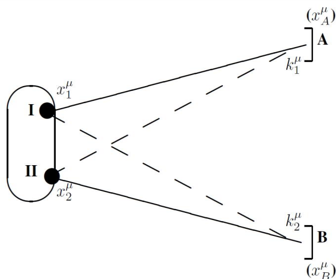
Figure 3. Simplified picture: two point sources, I and II, emit quanta considered as plane waves, which are observed in detectors A and B, respectively, with momenta k_1^\mu and k_2^\mu . Since the quanta are indistinguishable, there are two possible combinations for this observation, illustrated by the two continuous and the two dashed lines.
