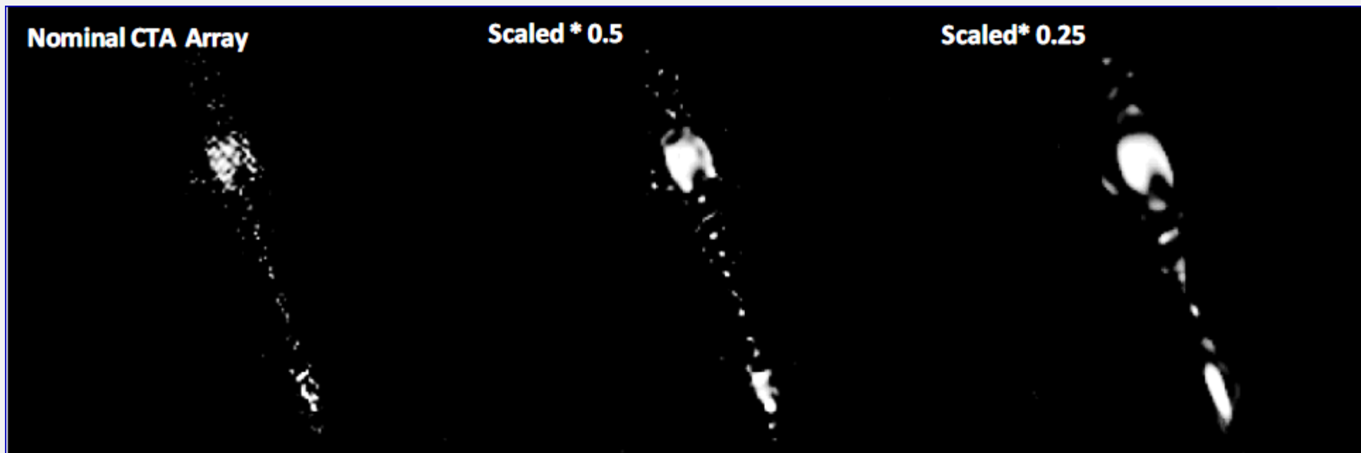
Image reconstruction of a geostationary satellite using a nominal CTA layout, and scaled versions
