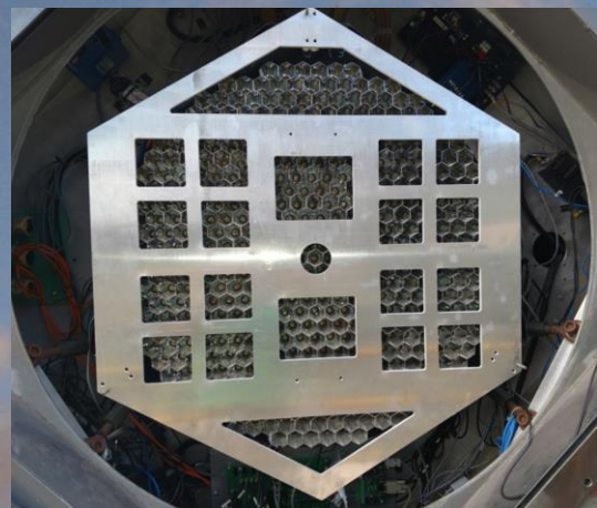
Camera baseplate for interferometry (David Kieda, Univ. of Utah, Sept. 2018)
