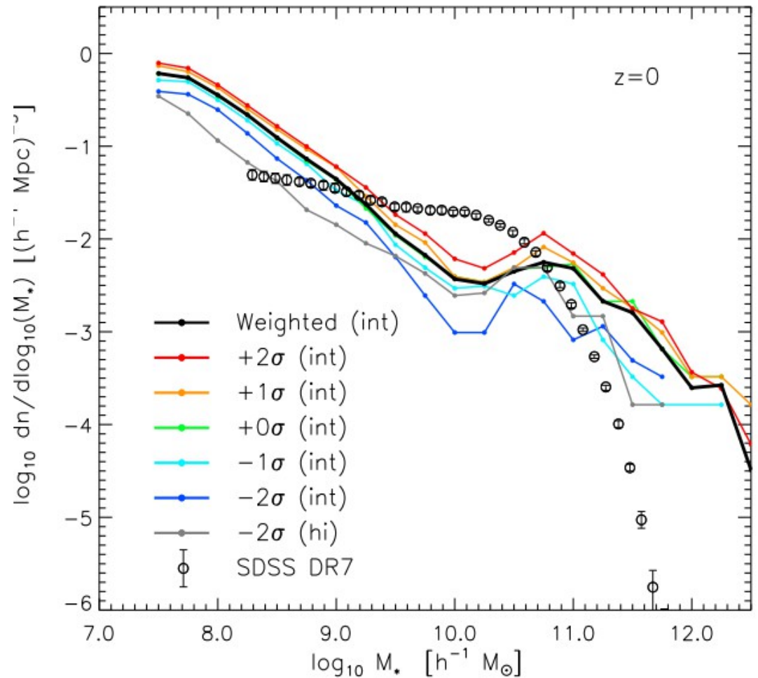
Crain et al. (2009)
