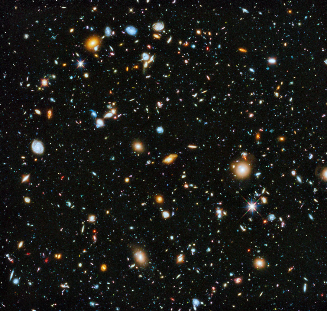
Hubble Ultra Deep Field
