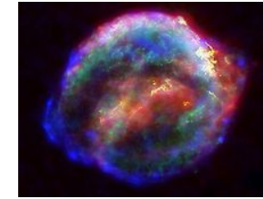
Kepler's Supernova
