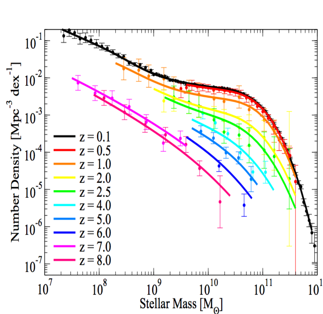
Behroozi, Wechsler & Conroy (2013)
