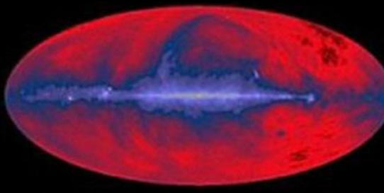
Radio 408\text{MHz} (C. Haslam et al., MPIfR, SkyView)
