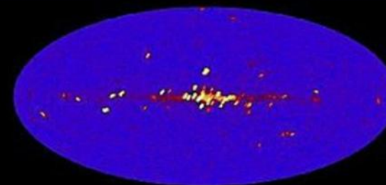
X-Ray 2-10\text{keV} (HEAO-1, NASA)
