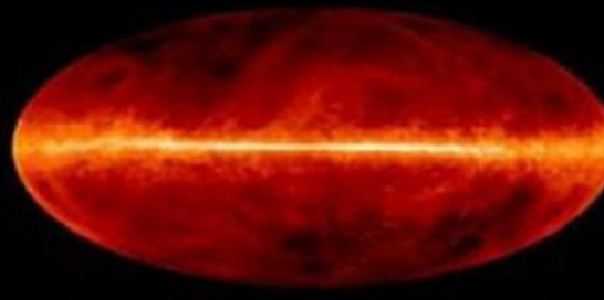
Radio 1420\text{MHz} (J. Dickey et.al. UMn. NRAO SkyView)
